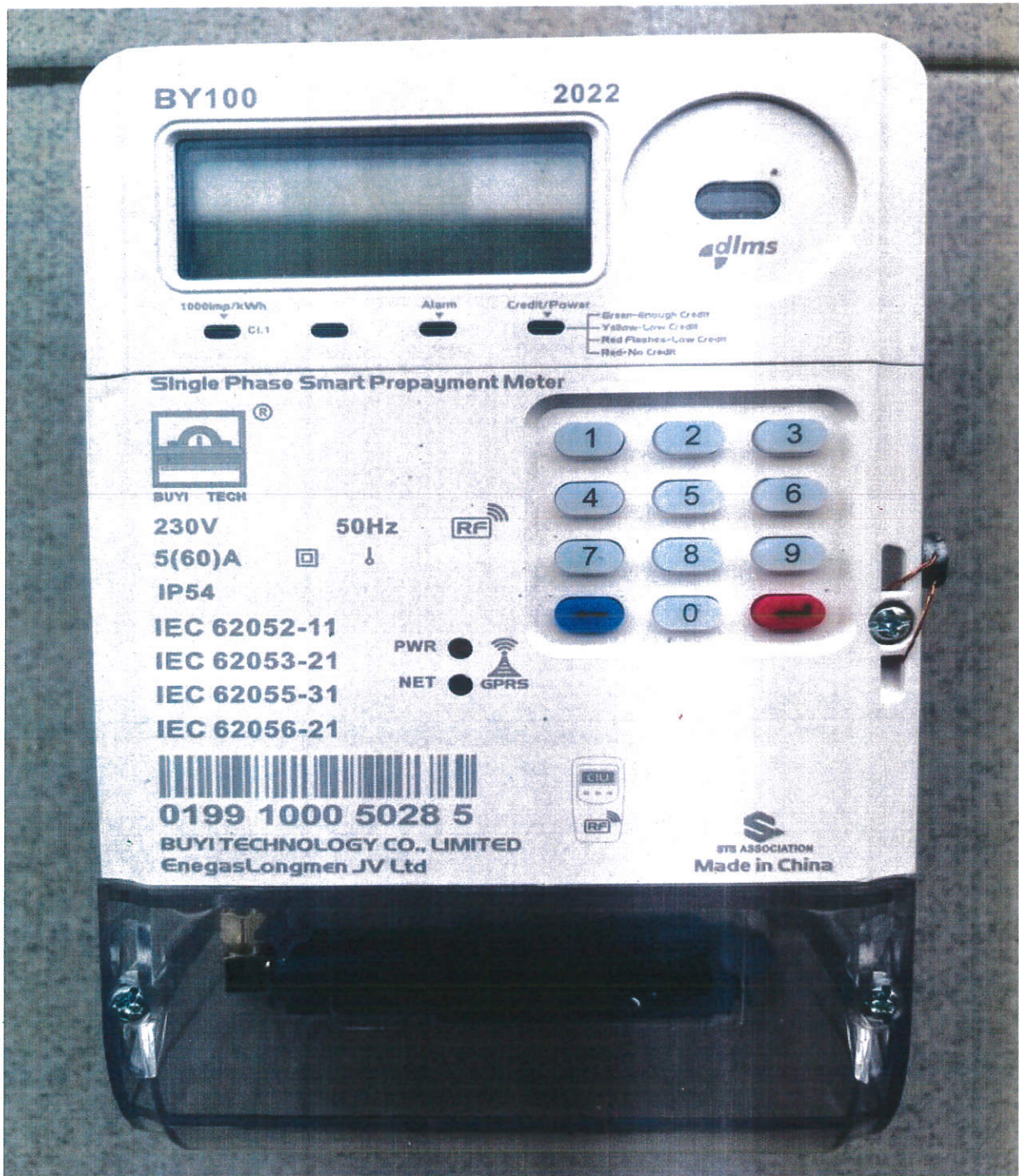
Above is a photograph of BUYI TECHNOLOGY CO. LTD & ENEGASLONGMEN JV LTD Single Phase Two Wire Smart Prepayment Energy Meter with extended terminal cover.
