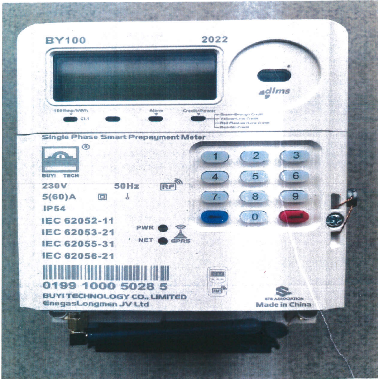
Above is a photograph of BUYI TECHNOLOGY CO. LTD & ENEGASLONGMEN JV LTD Single Phase Two Wire Smart Prepayment Energy Meter with terminal cover opened.
