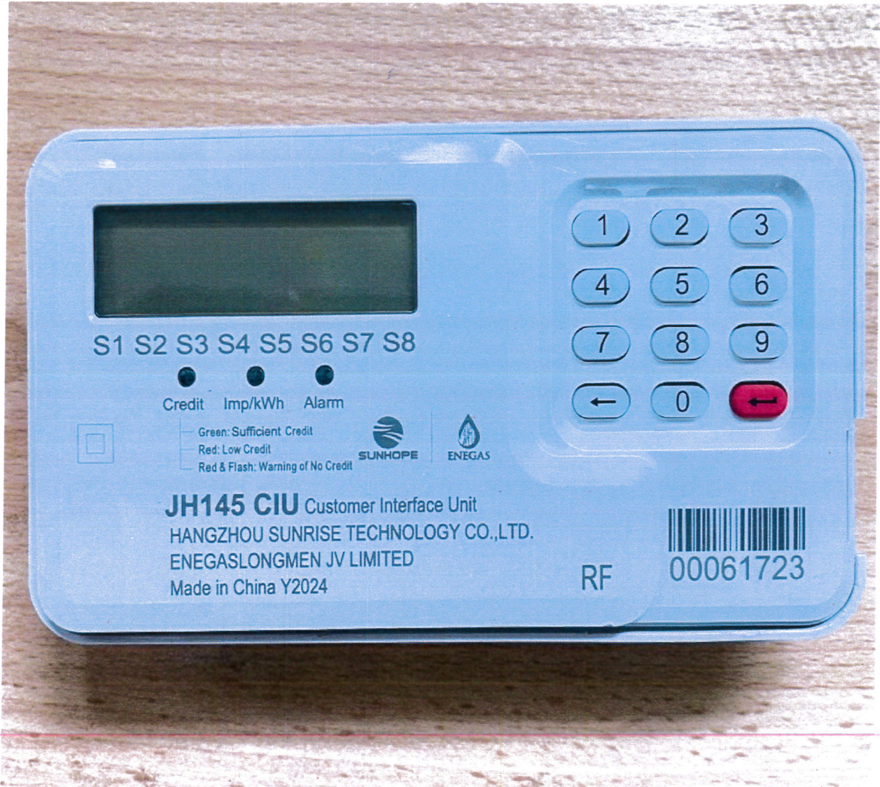
Photograph of HANGZHOU SUNRISE TECHNOLOGY CO., LIMITED & ENEGASLONGMEN JV LIMITED Single Phase Two Wire Smart Energy Meter Customer Interface Unit (CIU).
