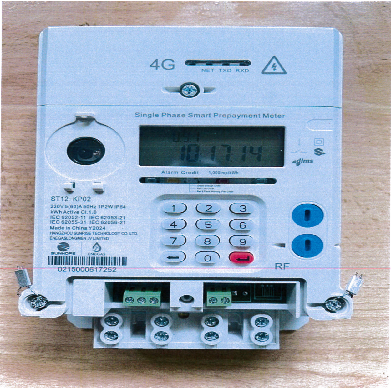
Photograph of HANGZHOU SUNRISE TECHNOLOGY CO., LIMITED & ENEGASLONGMEN JV LIMITED Single Phase Two Wire Smart Energy Meter with terminal cover open
